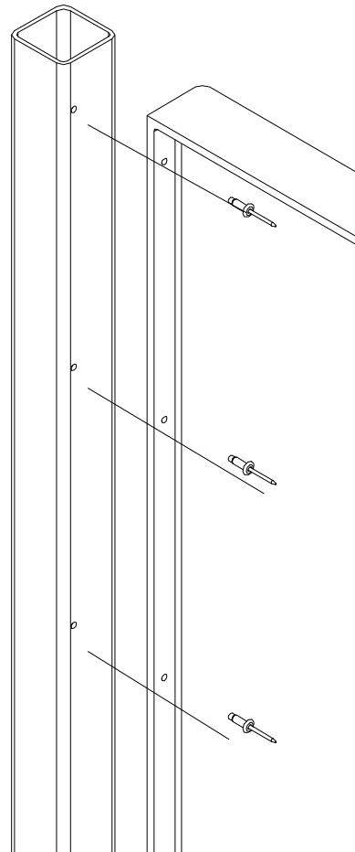
Assembly View
